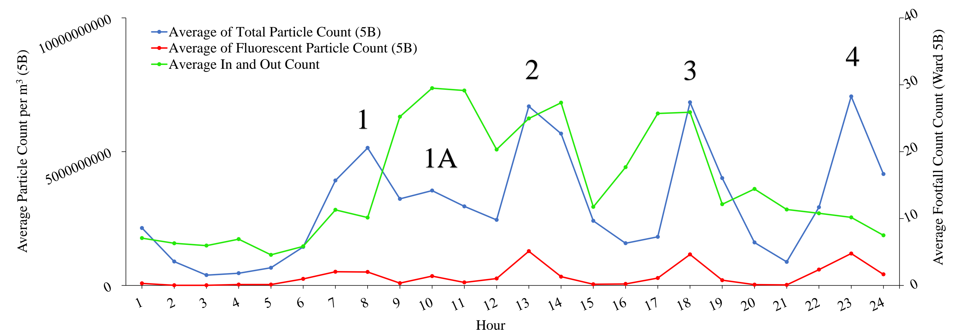
Fig 2.2 Average Diurnal Fluorescent Particle Count Ward 5B with Average Footfall Counts.
