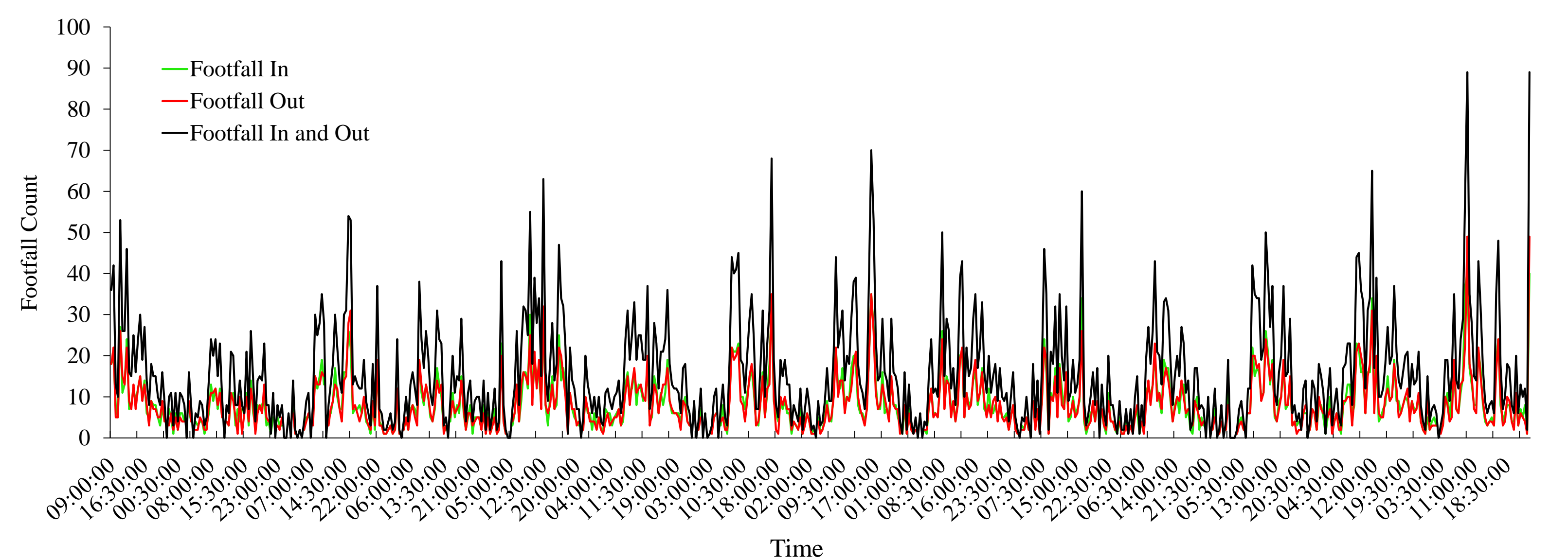
Fig 2.3 Time series of the week period with the colour key within indicating the Footfall in, out or total.
